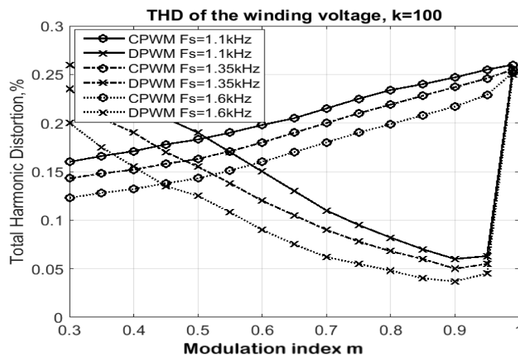
Figure 14. THD factor of the winding voltage of power transformer of grid-tied PV station as function of coefficient (index) of modulation m of dual VSDCI for different values of its SwF.
