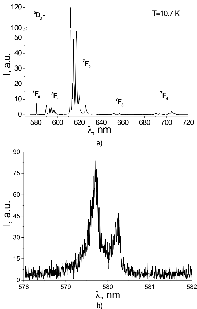
Figure 4. Low-resolution PL spectrum of the binuclear complex [\text{Eu}(\mu_2\text{-OC}_2\text{H}_5)(\text{btfa})(\text{NO}_3)(\text{phen})]_2 \cdot \text{phen} at 10.7 K [5] (a) and high-resolution spectrum of PL emission band ^5\text{D}_0 \rightarrow ^7\text{F}_0 ( \lambda_{\text{exc}} = 405 \text{ nm} ) (b).
