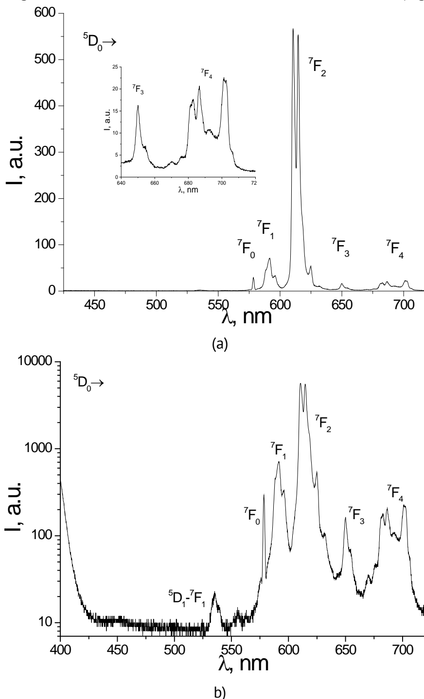
Figure 1. Low-resolution PL emission spectrum of the powder sample [Eu( \mu_2 -OC 2 H 5 )(btfa)(NO 3 )(phen)] 2 ·phen measured at 300 K under excitation 375 nm: a) linear and b) logarithmic scale.
