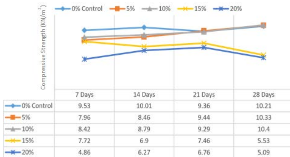
Figure 4. Compressive strength for % replacement of rice husk ash.
