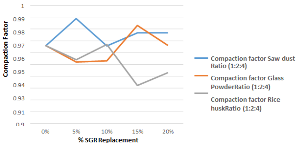
Figure 1. Compaction factor for saw dust ash, glass powder and rice husk ash.
