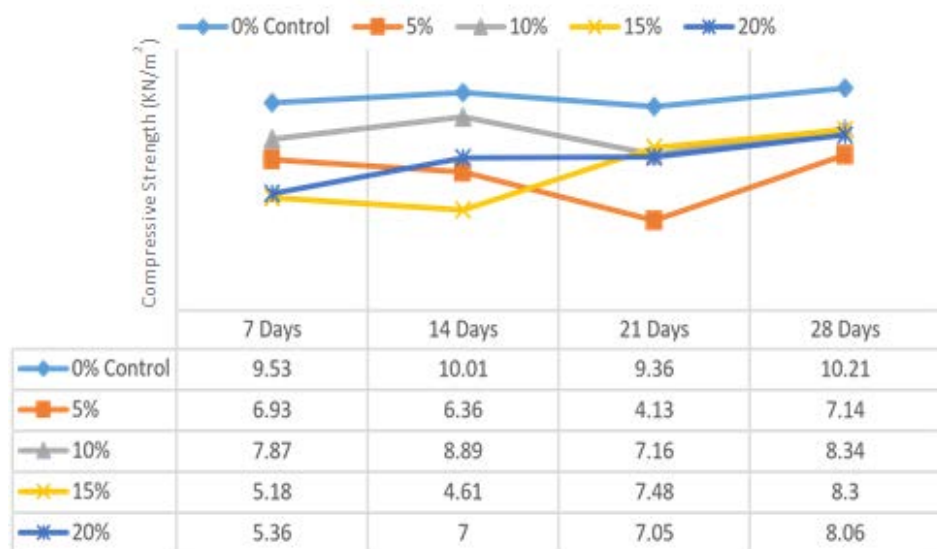
Figure 3. Compressive strength for % replacement with glass powder.
