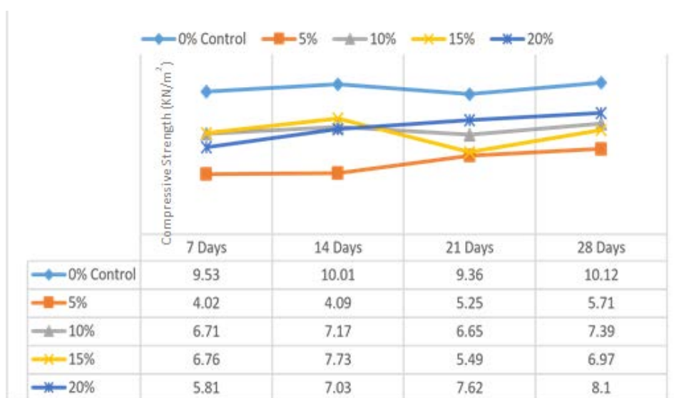
Figure 2. Compressive strength for % replacement with saw dust ash.
