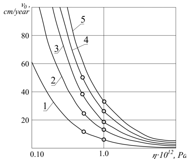
Figure 7. The graphs of dependence between speed of creep deformation ( v_0 ) and coefficient of viscosity ( \eta ) at different values of structural cohesion ( C_c ):
